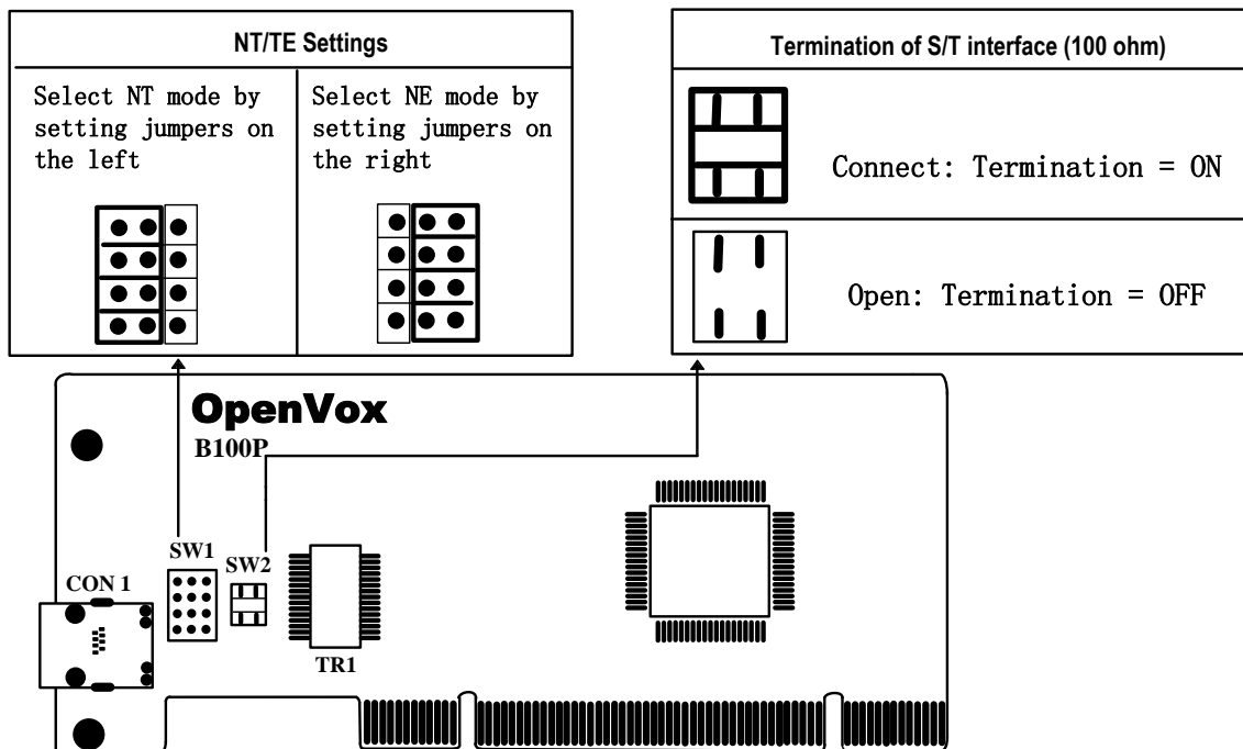
Figure 3 Jumper setting
