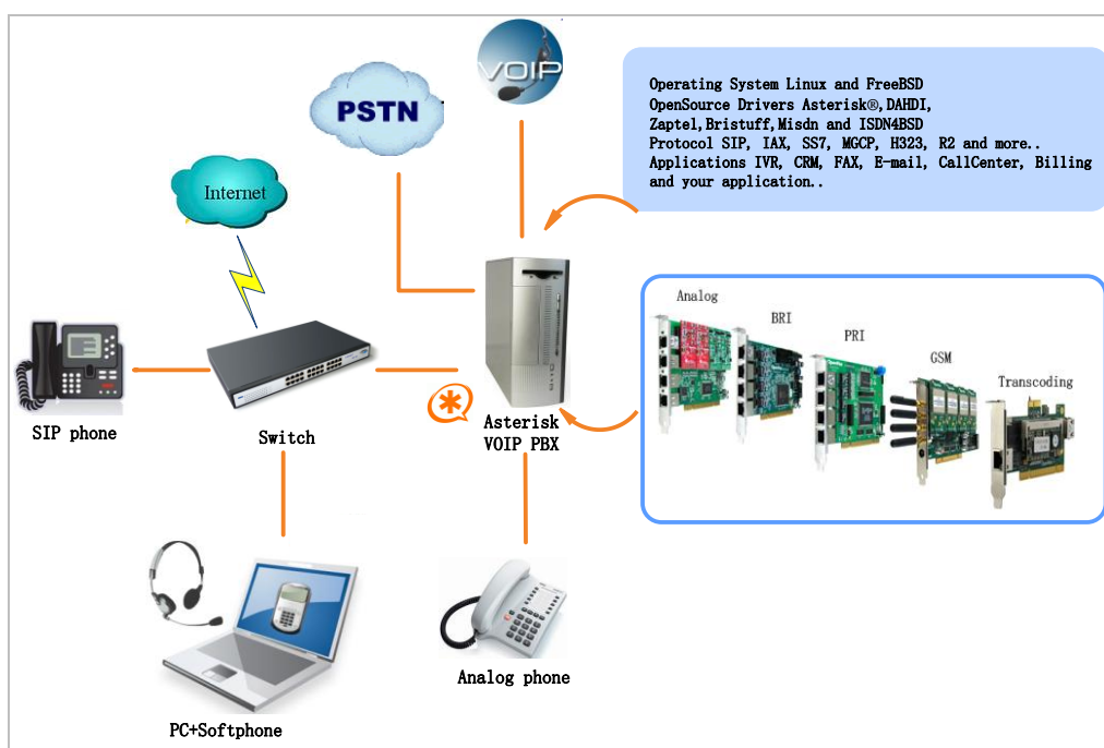
Figure 1 Topology
